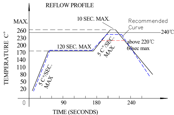
回流焊曲线图 Reflow soldering curve
