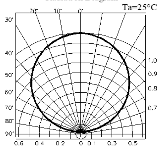
Radiation Diagram
