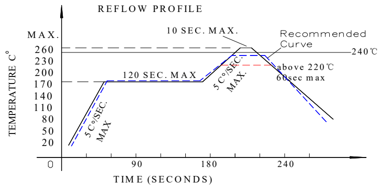
回流焊曲线图 Reflow soldering curve
