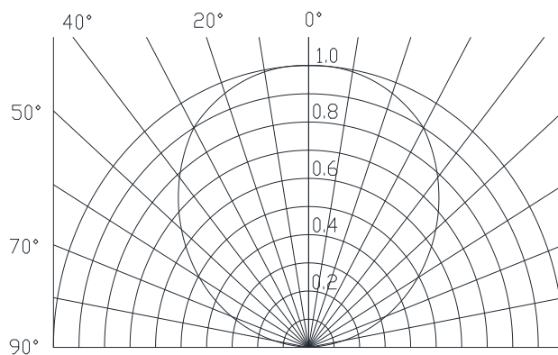
Curves of beam angle and relative brightness
