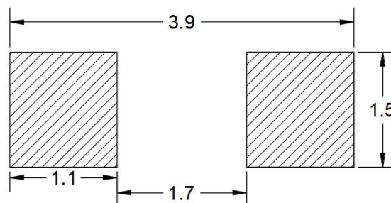
建议焊盘尺寸图 Recommended Soldering Pattern
